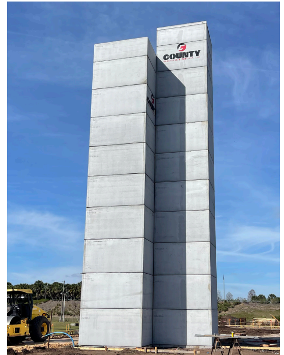
Stair Shaft
