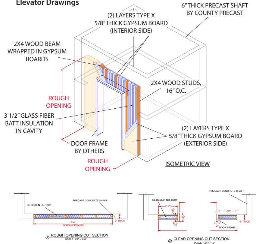
Elevator Shaft
