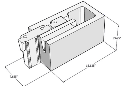
System 8 Right Corner Jamb
