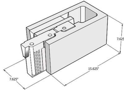
System 8 Left Corner Jamb
