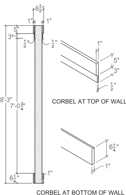
8' BLOCK WALL CORBEL DETAILS
