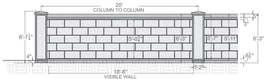
BLOCK WALL DESIGN (6' WALL SYSTEM)
