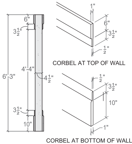
6' SMOOTH WALL CORBEL DETAILS
