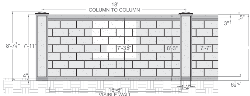
BLOCK WALL DESIGN (8' WALL SYSTEM)
