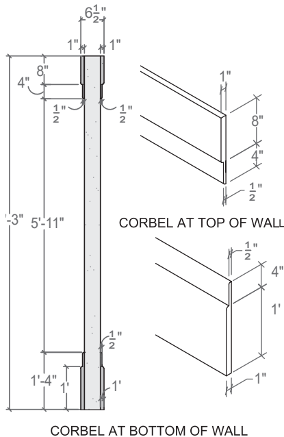
8' SMOOTH WALL CORBEL DETAILS
