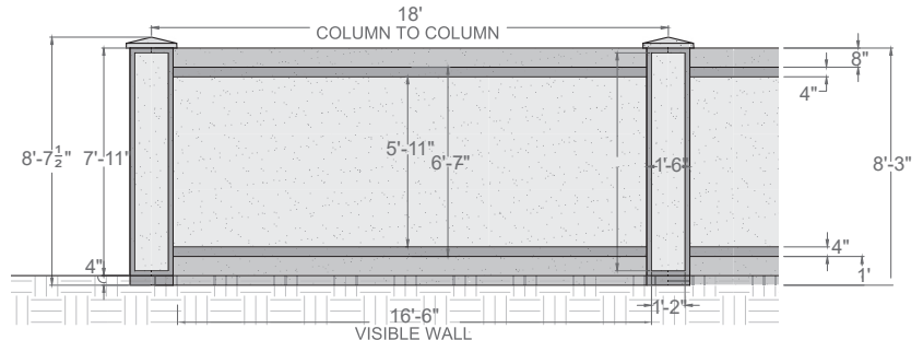
SMOOTH WALL DESIGN (8' WALL SYSTEM)
