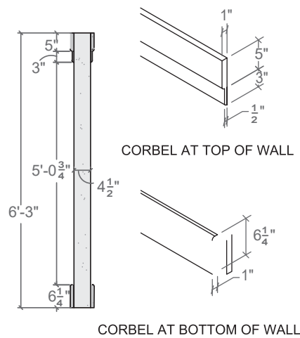
6' BLOCK WALL CORBEL DETAILS
