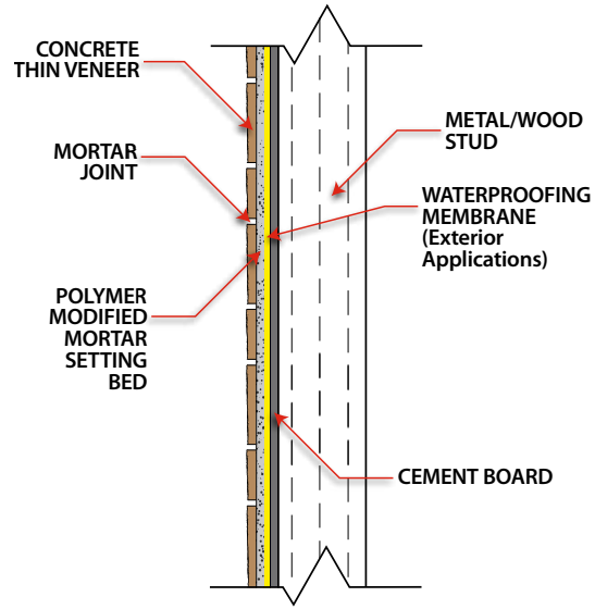
CONCRETE THIN VENEER ON CEMENT BOARD WITH POLYMER MODIFIED SETTING MORTAR (SIDE VIEW)
