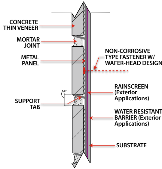
CONCRETE THIN VENEER ON METAL PANEL METHOD (SIDE VIEW)
