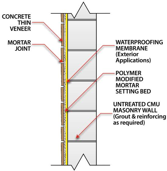
CONCRETE THIN VENEER ON CMU/MASONRY WALL (SIDE VIEW)
