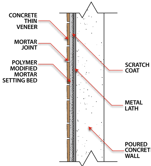
CONCRETE THIN VENEER ON POURED CONCRETE WALL (SIDE VIEW)
