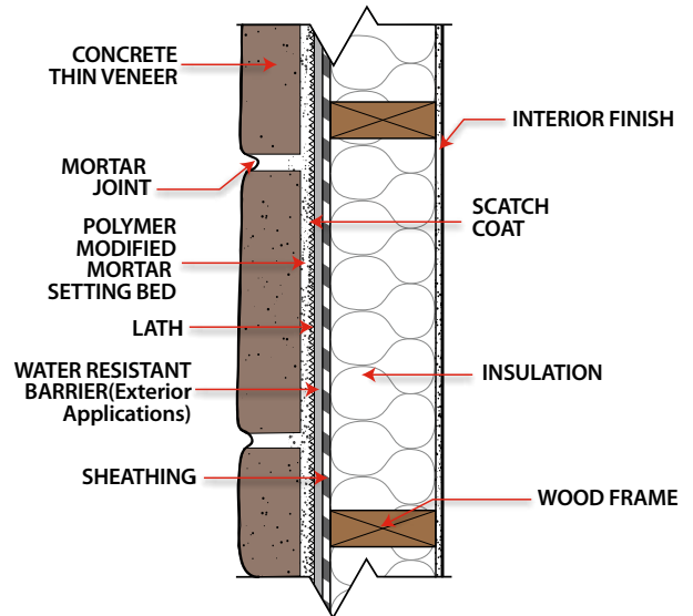
CONCRETE THIN VENEER ON WOOD FRAME W/SHEATHING (TOP VIEW)
