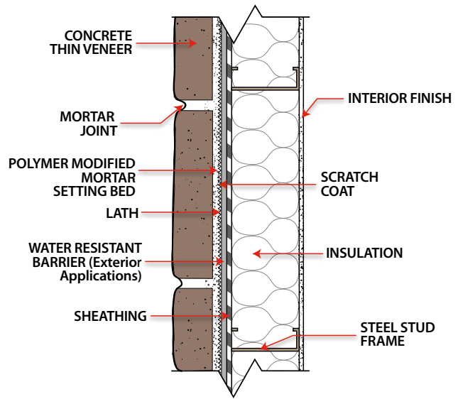
CONCRETE THIN VENEER ON STEEL STUD W/SHEATHING (TOP VIEW)
